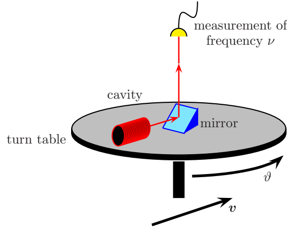
Figure 2. Basic setup for a cavity experiment testing the spatial isotropy and the independence of the speed of light from the velocity v of the laboratory. If SR is valid, then the measured frequency is independent of \vartheta and v .
