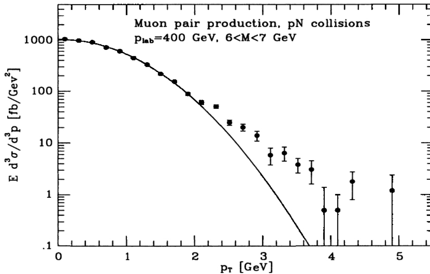
Fig. 9.2. The lepton pair transverse momentum from the CFS collaboration [4]. The curve corresponds to a Gaussian intrinsic k_T distribution for the annihilating partons.
