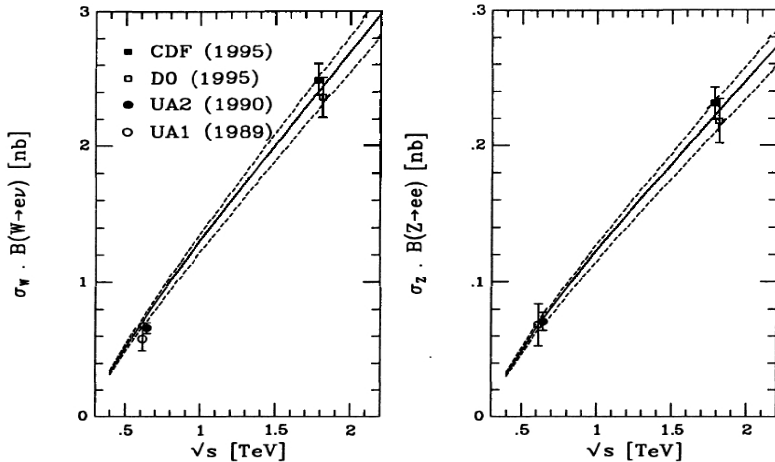
Fig. 9.6. Comparison of W and Z cross section measurements in p\bar{p} collisions with theoretical predictions. The systematic and statistical errors on the measurements have been combined in quadrature.
