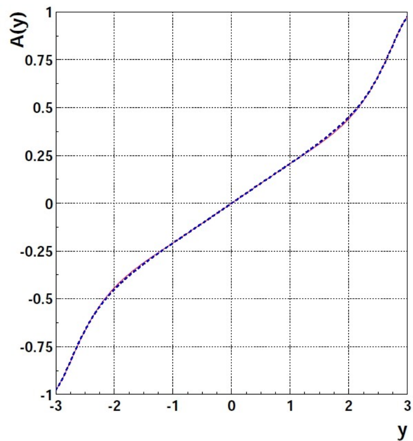
W asymmetry
