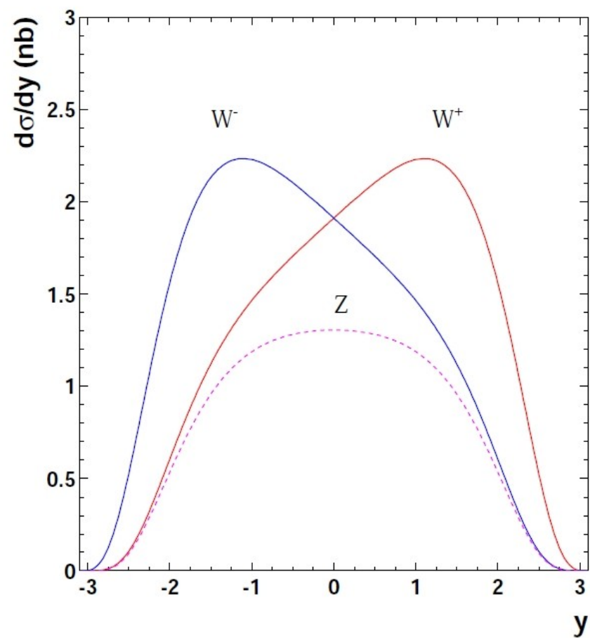
W and Z production cross sections
