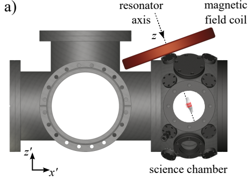
Figure 5.8: Guiding magnetic field: a) Position of the field coil at the science chamber. The axes of the coil and the resonator are parallel. b) Magnetic field parallel ( B_z , blue) and normal ( B_{\text{normal}} , red) to the resonator axis. The position of the resonator is approximately at z = 0 . This region is magnified in the inset where the dashed lines assume a displacement of \pm 20 mm along x' between the resonator and the coil axis.
