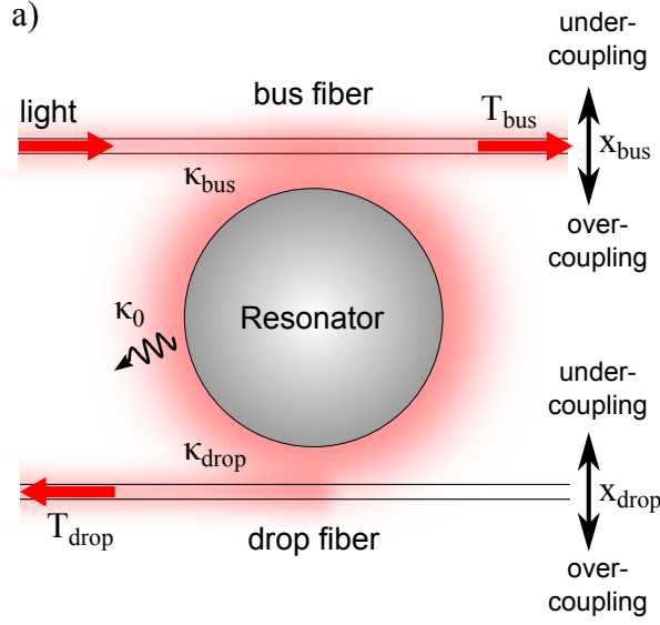
Figure 3.11: a) Schematic of two ultra-thin fibers coupled to a WGM resonator in the add-drop configuration. b) On-resonant bus fiber transmission T(0, x_{\text{bus}}) as function of x_{\text{bus}} for a fixed x_{\text{drop}} : When the bus fiber is critically coupled to the combined resonator–drop fiber system, a reduction of the bus fiber–resonator gap x_{\text{bus}} brings the system into over-coupling while an increase of x_{\text{bus}} under-couples the system. c) In contrast, a change of the drop fiber–resonator gap x_{\text{drop}} has the inverse effect on the bus fiber transmission. Parameters of the plots are \kappa_0/2\pi = 5 MHz, a) \kappa_{\text{drop}}/2\pi = 20 MHz, \kappa_{0,\text{bus}} = /2\pi = 25 MHz, and b) \kappa_{\text{bus}}/2\pi = 25 MHz, \kappa_{0,\text{drop}} = /2\pi = 20 MHz.
