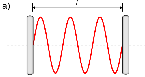
Figure 2.1: a) Working principle of the Fabry-Pérot interferometer which confines light between two parallel mirrors. When the separation l of the mirrors is an integer multiple of a half-wavelength \lambda/2 a standing wave can build up in the resonator. b) Intra-cavity intensity of a Fabry-Pérot resonator as function of the light frequency \nu . The spectrum is calculated from Eq. (2.3) for three different values of finesse: F = 5 (blue), F = 10 (red) and F = 100 (green).
