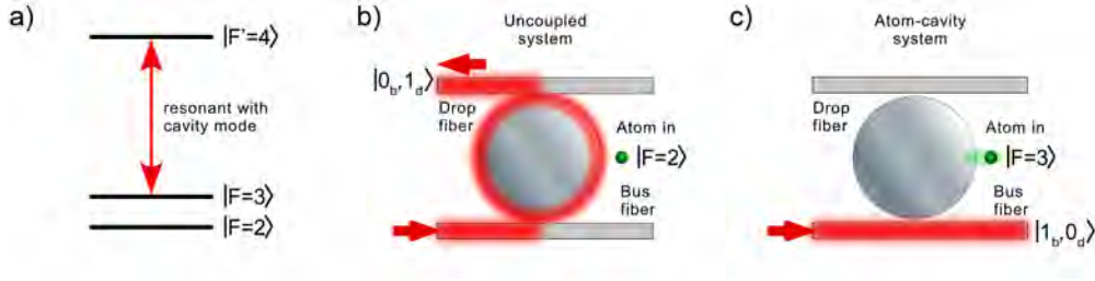
Figure 6.7: Concept of the optical switch controlled by the internal state of the atom. a) Relevant states of a three-level atom where only one of the two possible transitions is resonant with the cavity mode. b) Since the |F = 2\rangle \rightarrow |F' = 4\rangle transition is off-resonant the presence of the atom does not alter the resonance condition of the optical switch and a single photon is transferred to the drop fiber ending up in the state |0_b, 1_d\rangle . c) An atom in the |F = 3\rangle state couples to the resonator and thereby blocks the build-up of an intra cavity field leaving an incoming photon in the state |1_b, 0_d\rangle .
