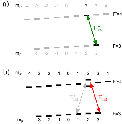
Figure 5.27: Modeling of the coupling between the E_{\text{TM}}^- mode and the atom in the m_F = +3 ground state. a) Level scheme of the ^{85}\text{Rb} D 2 line where only the levels |F = 3, m_F = 3\rangle and |F' = 4, m_{F'} = 2\rangle are taken into account for the modeling of the interaction between the E_{\text{TM}}^- mode and the atom. b) Taking into account the full multi-level structure of the atom for the modeling, the coupling to the empty E_{\text{TM}}^+ mode induces a vacuum-Rabi splitting of the excited m_F = +2 state (Note that also all other excited state have a vacuum-Rabi splitting which is left out here for clarity). c) Data from Fig. 5.26 c) (blue points) and simulated spectra for the modeling in a) and b). The spectra are averaged over a distribution of the coupling strength g as explained in the text.
