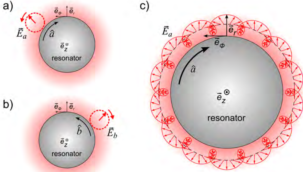
Figure 4.12: a) TM polarized mode propagating clockwise in the WGM microresonator. The red arrows illustrate the rotation sense of the nearly circular polarization of the evanescent field. b) Same as a) but for a counter-clockwise propagating TM mode. c) The polarization vector of the evanescent field describes a cycloid along the circumference of the resonator in the case of perfect circular polarization ( |E_{\text{long}}/E_{\text{trans}}| = 1 ).
