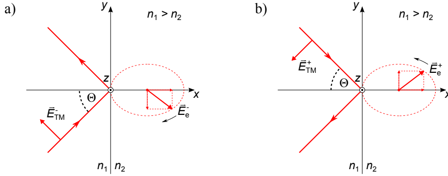
Figure 4.6: Total internal reflection of a TM polarized wave \vec{E}_{\text{TM}}^\pm at the interface to an optical thinner medium. The propagation of the evanescent wave along the interface is in the a) positive and b) negative y -direction. In the second medium ( x > 0 ) the polarization state of the evanescent field \vec{E}_e^\pm = E_{\text{trans}}\vec{e}_x \pm iE_{\text{long}}\vec{e}_y is illustrated, where the rotation sense of the elliptical polarization depends on the propagation direction of the incoming wave. Figures follow Refs. [48, 112].
