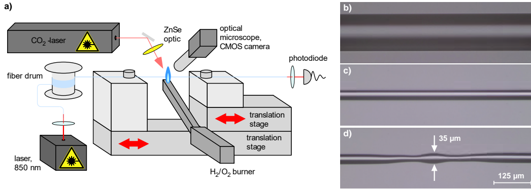
Figure 2.4: a) Schematic of the fiber pulling rig used for the fabrication of bottle microresonators and ultra-thin fibers. In order to heat the fiber, either an oxygen-hydrogen flame or a focused beam of a CO 2 -laser is used. The fiber is clamped onto two translation stages, which allow one to translate and stretch the fiber. The fiber pulling process is monitored in real-time with an optical microscope and via the transmission of a laser with a wavelength of 850 nm through the fiber. b)-d) Microscope images of the bottle microresonator fiber in the pulling rig at different processing steps. b) Unprocessed fiber with a diameter of 125 μm. c) Central part of the tapered fiber with a diameter of 35 μm. d) Tapered fiber after micro-structuring with the CO 2 -laser. The central bulge is the bottle microresonator. Figures adapted from Ref. [53].
