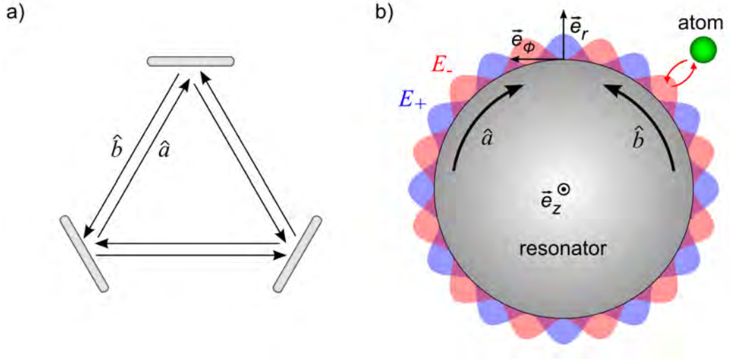
Figure 4.4: a) Simple model of a three-mirror ring cavity with two degenerate, scalar light waves \hat{a} and \hat{b} , propagating clockwise and counter-clockwise, respectively. b) Equivalent description of a WGM resonator as ring cavity. The superposition of the two scalar running waves \hat{a} and \hat{b} creates two standing waves \hat{u}_+ and \hat{u}_- , which are spatially shifted against each other by \pi/2 . The phase of the standing wave pattern can always be chosen such that the atom couples only to one of the standing waves.
