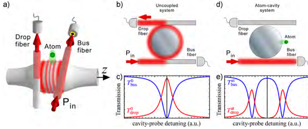
Figure 6.1: Concept of the optical fiber switch based on the bottle resonator. a) Two fibers are coupled to the bottle resonator in add-drop configuration. To control the light flux between the bus and the drop fiber a single atom is broad in the evanescent resonator field. b) Uncoupled system: The bus fiber is critically coupled so that the complete incoming light power P_{in} is transferred into the resonator from where it couples to the drop fiber. c) Corresponding spectrum of the system with the bus and drop fiber transmissions T_{bus}^0 (blue) and T_{drop}^0 (red). d) Coupled system: The atom blocks the build-up of an intra-cavity field and the light remains in the bus fiber. e) Corresponding transmission spectrum showing the vacuum-Rabi splitting of T_{bus}^{at} and T_{drop}^{at} which prevents the build-up of an intra-cavity field on resonance. Figures appeared in Ref. [111].
