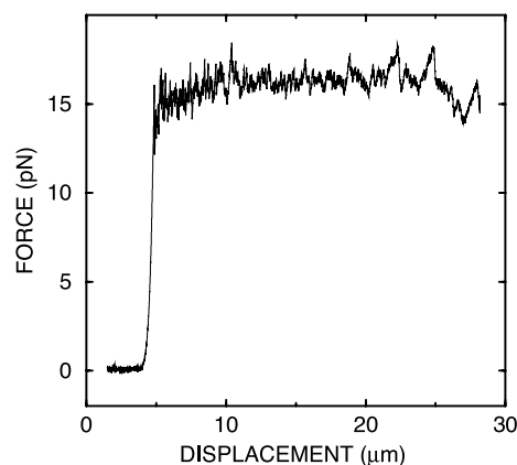
FIGURE 11 Force versus displacement curves corresponding to mechanical unzipping of a single \lambda -phage DNA molecule. The trace is recorded during opening of the double helix with a constant displacement velocity of 1 \mu\text{m/s} (sampling rate of 400 Hz, aliasing filter cutoff frequency of 176 Hz).
