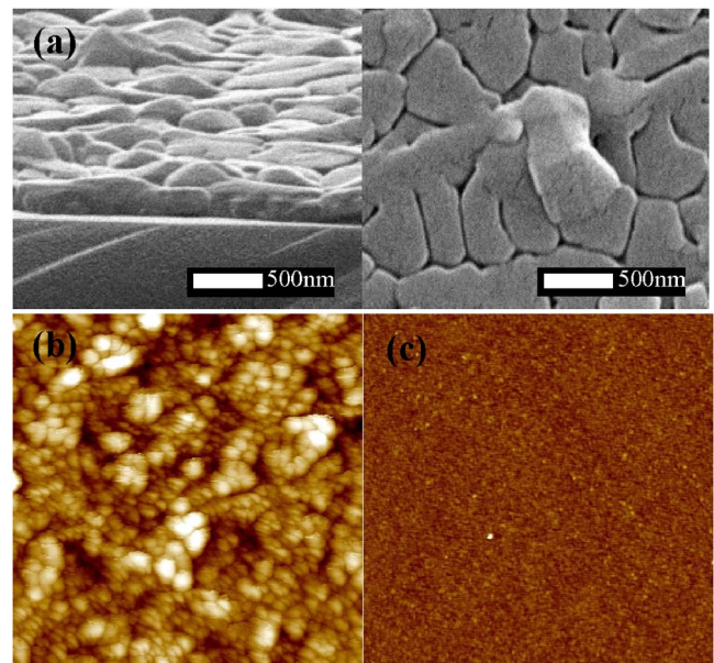
FIG. 3. (Color online) (a) SEM section view (left) and top view (right) micrographs of pentacene/oxidized Si. (b) AFM micrograph of ITO and (c) oxidized Si (both AFM images, 1 \times 1 \mu\text{m}^2 ; height-scale, 10 nm for ITO and 2 nm for oxidized Si).
