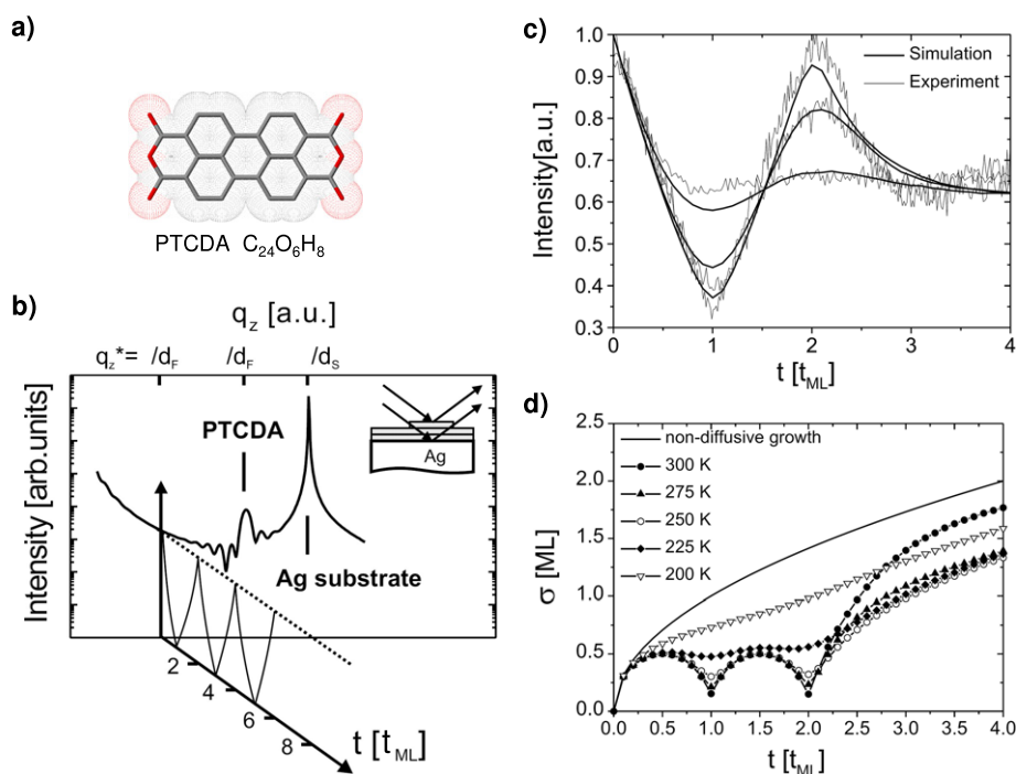
Figure 8. (a) Schematic of the molecule 3,4,9,10-perylenetetracarboxylic dianhydride (PTCDA). (b) Simulation of the specular reflectivity of a PTCDA film on an Ag (111) substrate (from [70]). At the anti-Bragg point of the PTCDA film ( q^*z = \pi/d_F ), the scattering of subsequent layers interferes destructively, so that during film growth the reflected intensity at the anti-Bragg point oscillates as a function of the deposition time. (c) Comparison between experimental anti-Bragg oscillations (substrate temperatures 233, 303, and 358 K) and Monte Carlo simulations (simulations at 200, 225, 250 K). (d) Interface roughness as obtained from Monte Carlo simulations at different temperatures. Clearly a transition from 2d to 3d growth is visible after two monolayers at high temperatures, which for low temperatures (200 K) occurs as early as after half a monolayer deposition. Reprinted figures with permission from [70].
