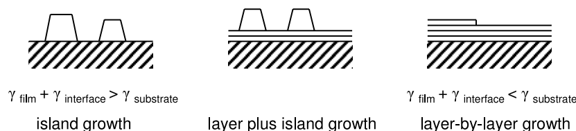
Figure 2. Scenarios for thin film growth: depending on the material specific surface free energies three different generic growth modes are generally distinguished: island growth, layer plus island growth, and layer-by-layer growth.
